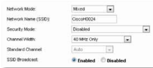
Basic Wireless Settings (Manual) > Wireless Settings
